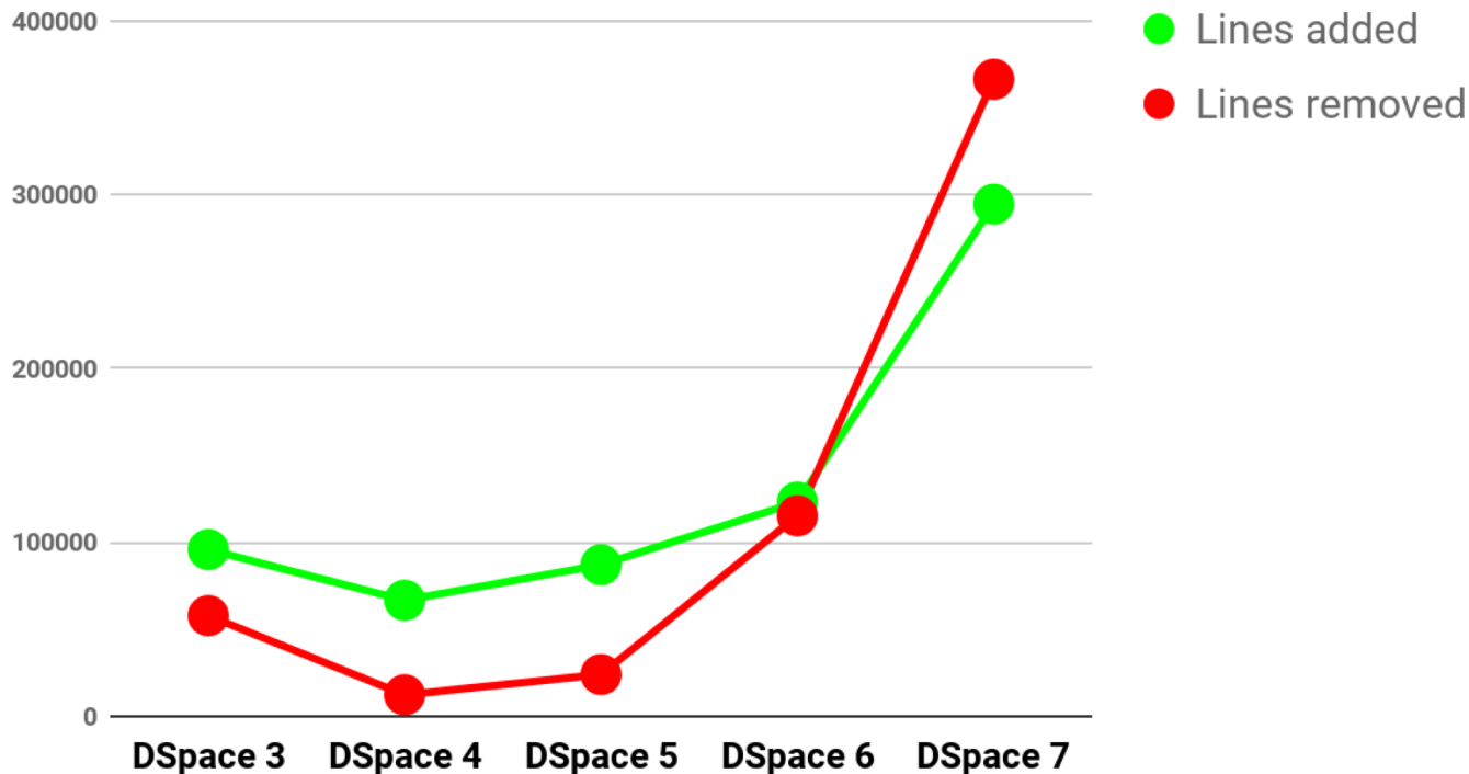
Lines of Code Changed per Major Release
